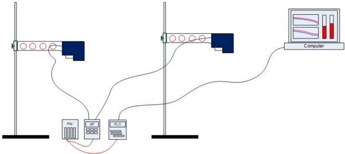
Figure 1: Schematic diagram of the Automatic display of the pistons floating position using laser displacement which operating with portable computer control and a floating position monitoring software
